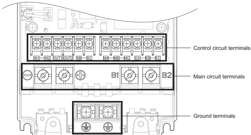
Figure 17 Wiring the Terminals
