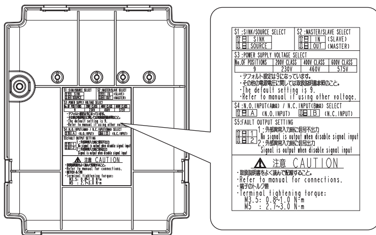
Figure 28 Switch Layout
